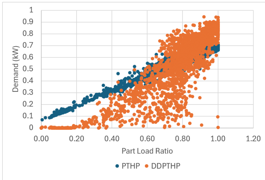
Figure 14: Site 2 PTHP vs. DDPHP power across site part load ratio.
