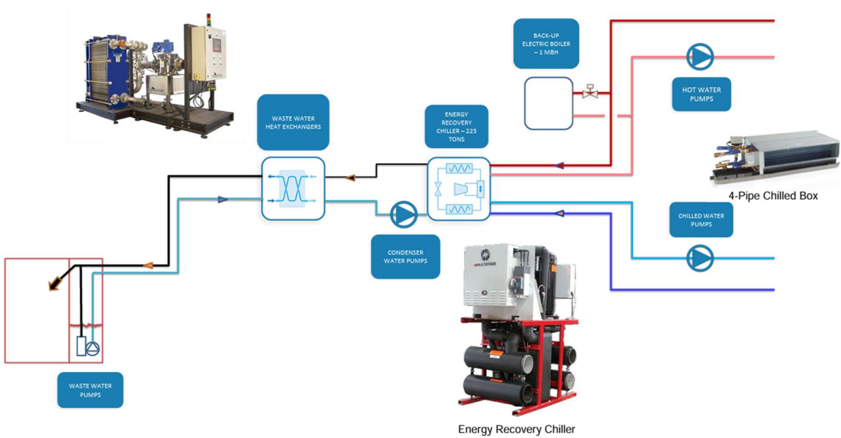
Figure 14: WET system schematics for D.C. Water Administrative Building.
