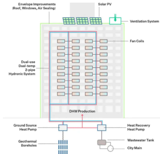
Figure 11: Amalgamated Housing Cooperative Towers WET retrofit.
