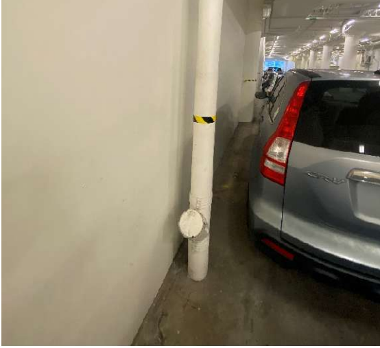
Figure 26: One of four sewer risers in Commercial Office Building A parking garage.
