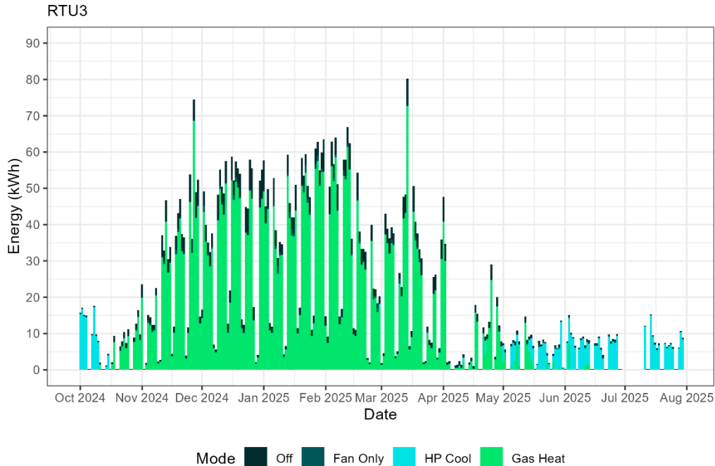
Figure 20. Gas-Fired RTU –Energy input by day and mode
