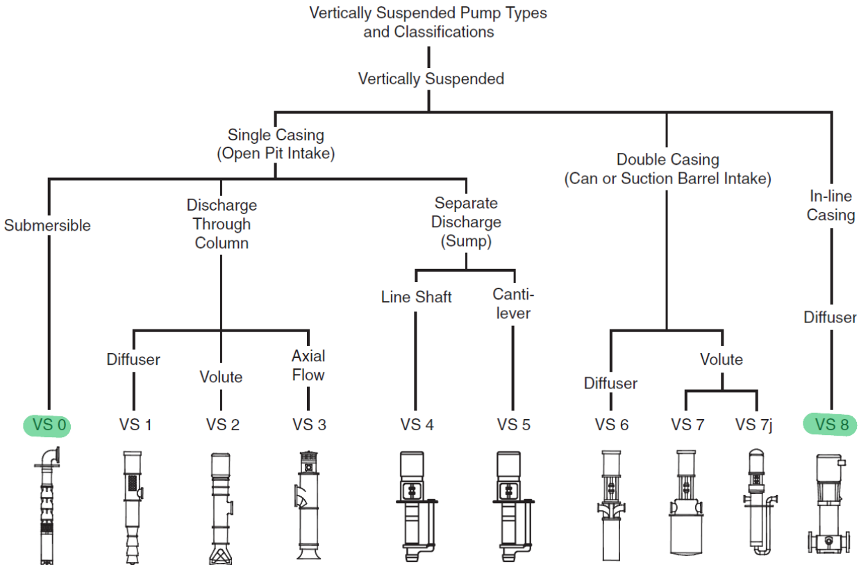
Figure 10: Rotodynamic vertically suspended pump types and classifications.
