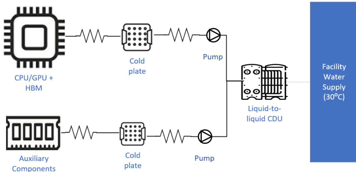
Figure 6: D2C liquid cooling with cold plates for all components.
