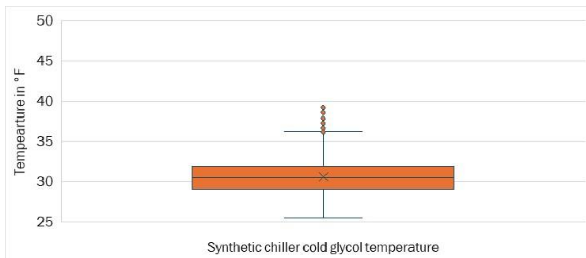
Figure 32: Cold glycol temperature during Synthetic Lead mode.
