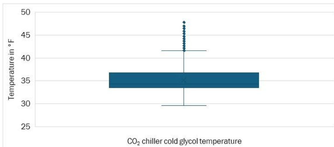
Figure 31: Cold glycol temperature during CO 2 Lead mode.
