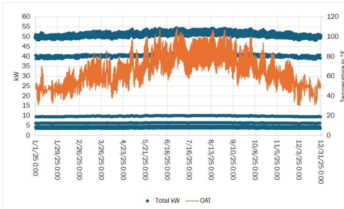
Figure 45: Normalized eastside chiller model using bin method.
