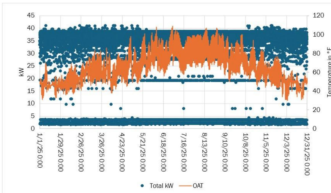
Figure 42: Normalized westside chiller model using array method.
