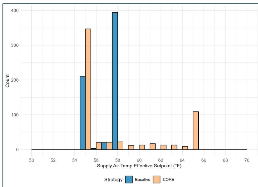
Figure 32: Supply air temperature setpoint distribution for Baseline and CORE—RTU 1—MOB-2.
