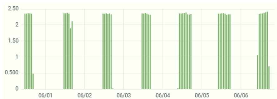
Figure 28: Daily leafy greens greenhouse supplemental lighting electricity consumption.
