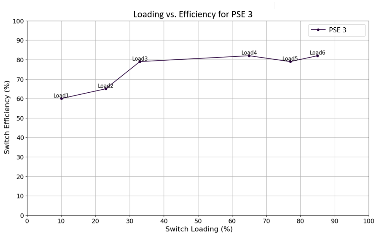
Figure 30: PSE 3 24 Port - Loading vs Efficiency
