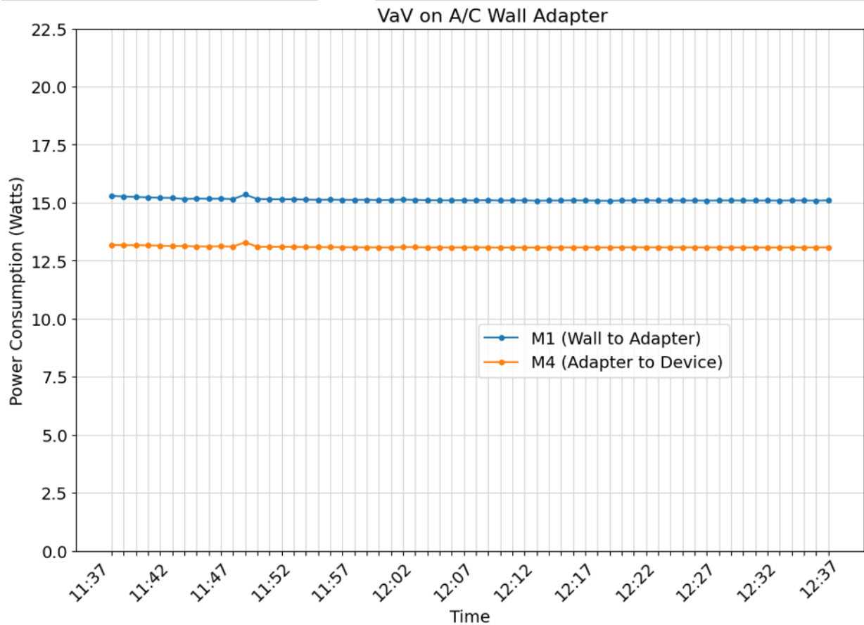
Figure 14. Power consumption of VaV Controller when powered by AC
