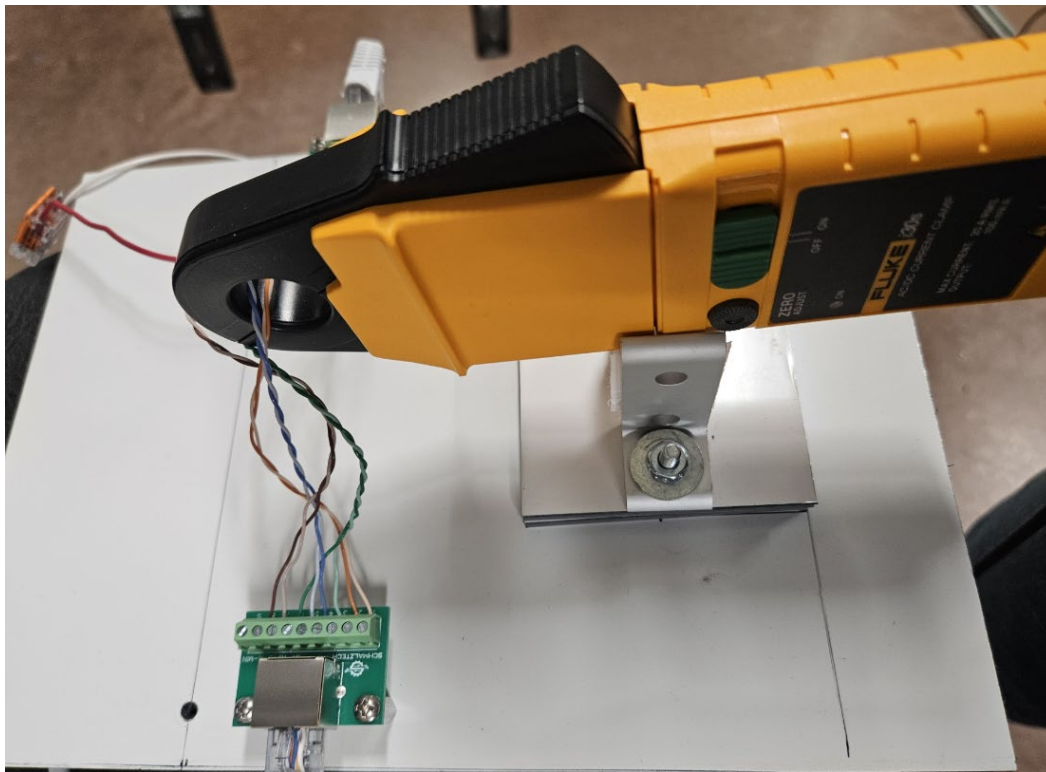
Figure 4: Fluke CT with Ethernet cable conductors passed through.
