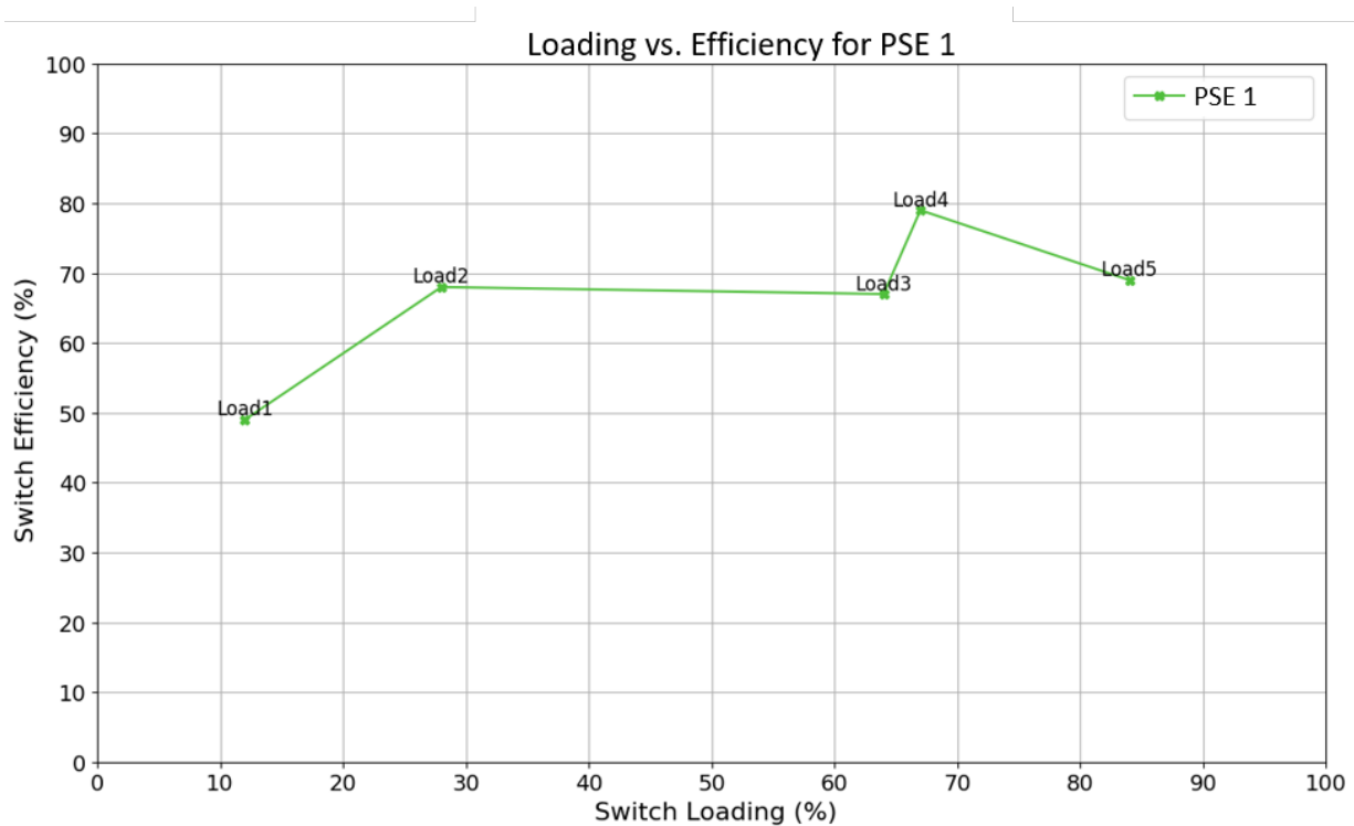
Figure 26: PSE 1 - loading vs. efficiency.
