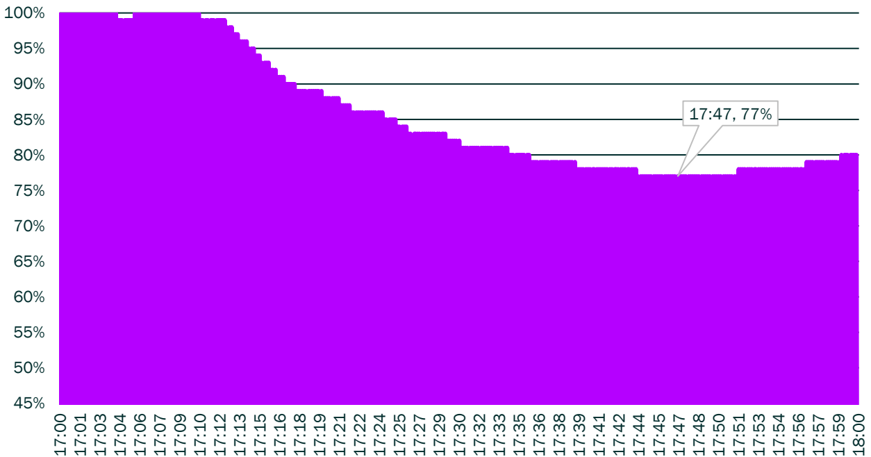
Figure 16: State of charge over time for the peak cooking event showing the depth of discharge the battery experienced through the event.
