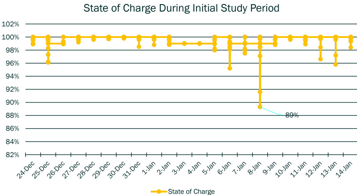
Figure 26: Battery state of charge over the initial prototype data collection period (22 days).
