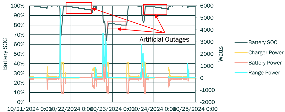
Figure 12: Time-series data for Stove 17, showing the battery state of charge and power during a series of temporary outages.
