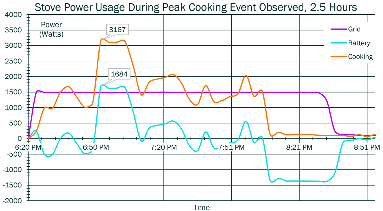
Figure 3: From the prototype unit: stove power at three different points: the grid, the battery, and the cooking elements.
