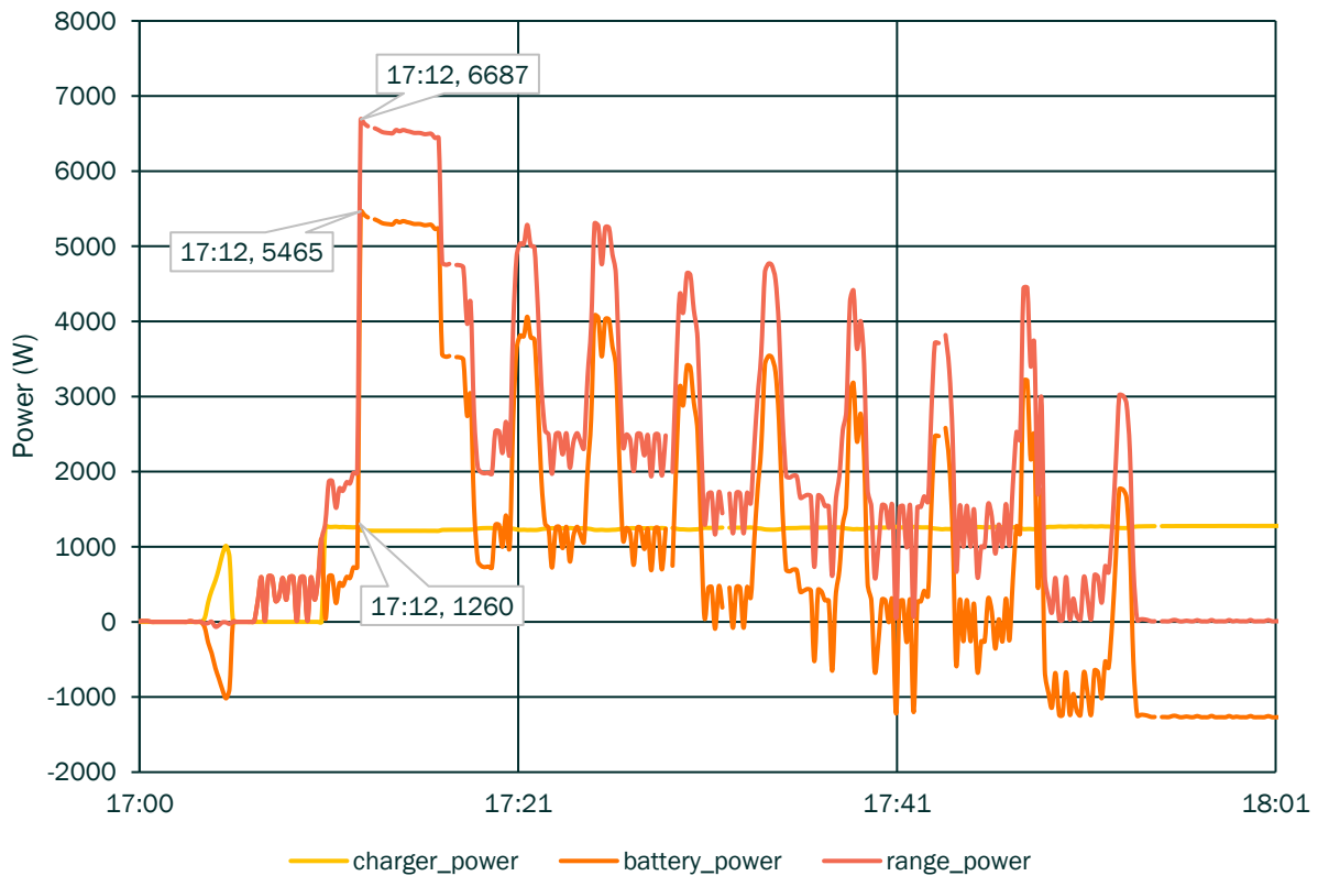
Figure 14: Time-series data highlights the most power-intensive cooking event observed.
