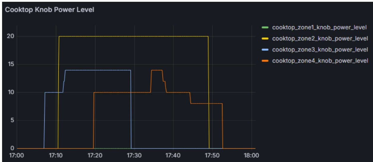
Figure 15: Breakdown of the position each stovetop element was set to during the peak cooking event.
