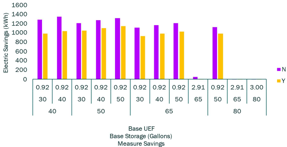
Figure 1: Average kWh savings for SWWH014 HPWH residential measure (3.5 UEF).
